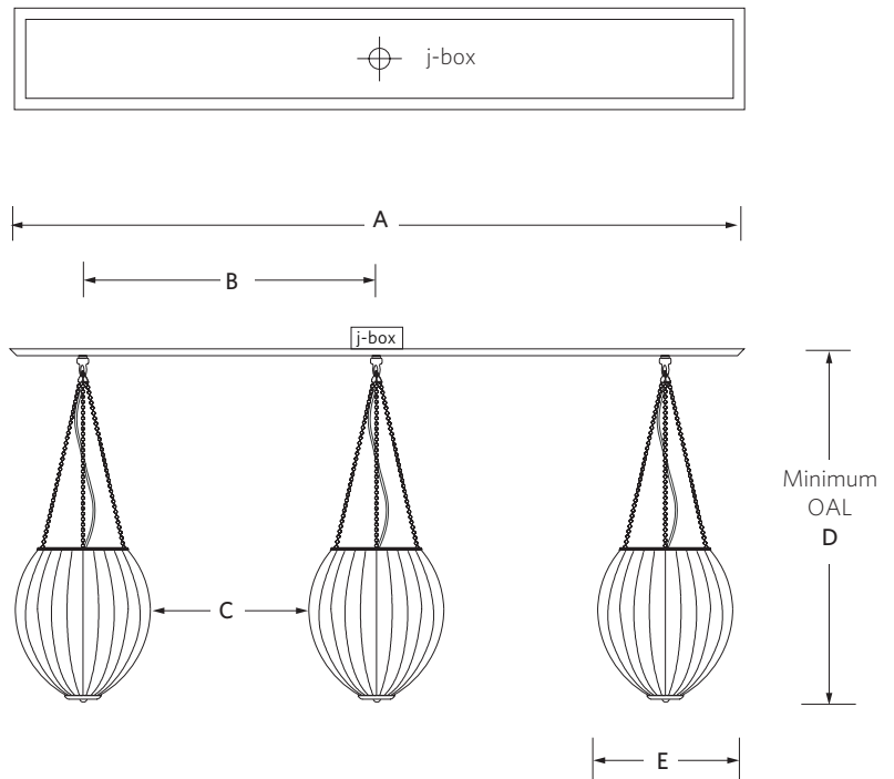
ceiling plate top view
