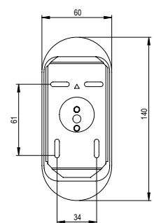
WALL BRACKET*
